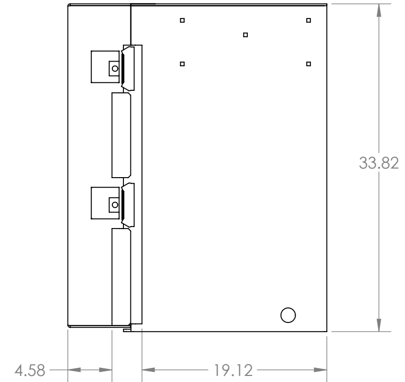
RIGHT SIDE
